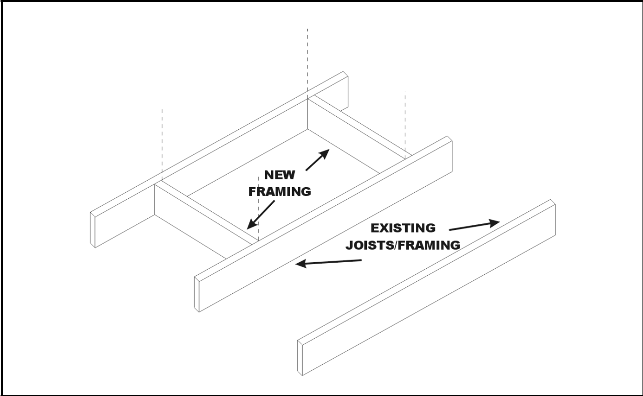
FIGURE 4 – Framing.
