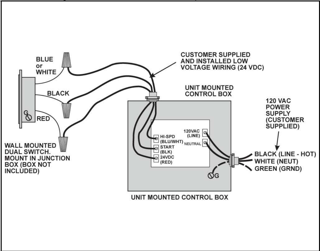
FIGURE 8 – Wiring with hardwired switch and hardwired power.
