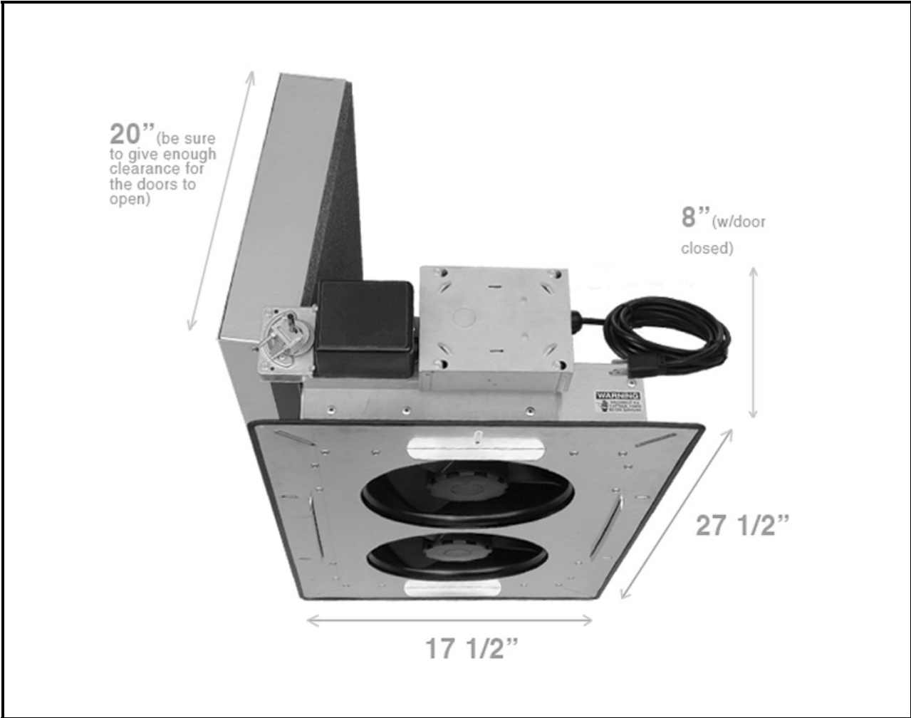
FIGURE 3 – Dimensions.
