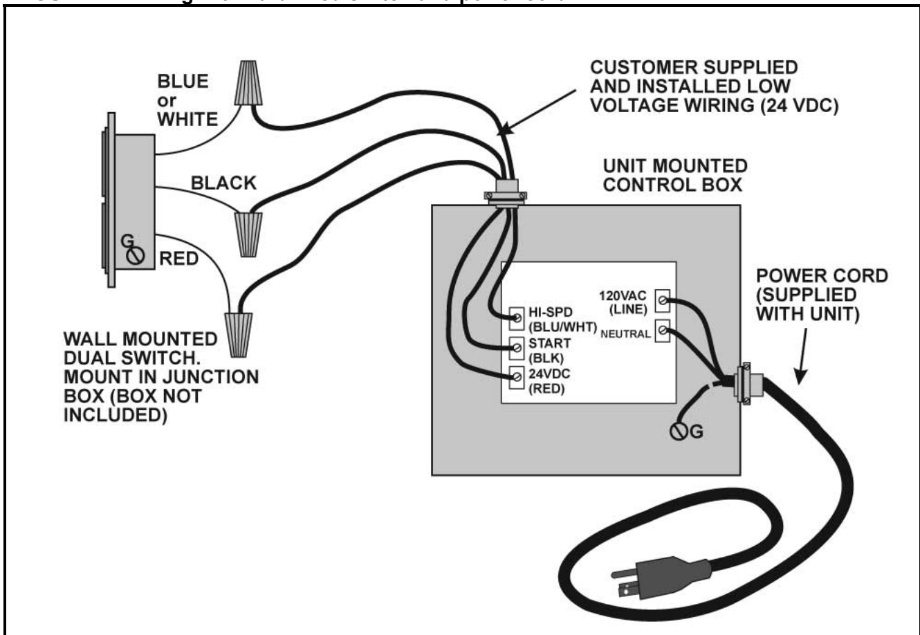
FIGURE 7 – Wiring with hardwired switch and power cord.
