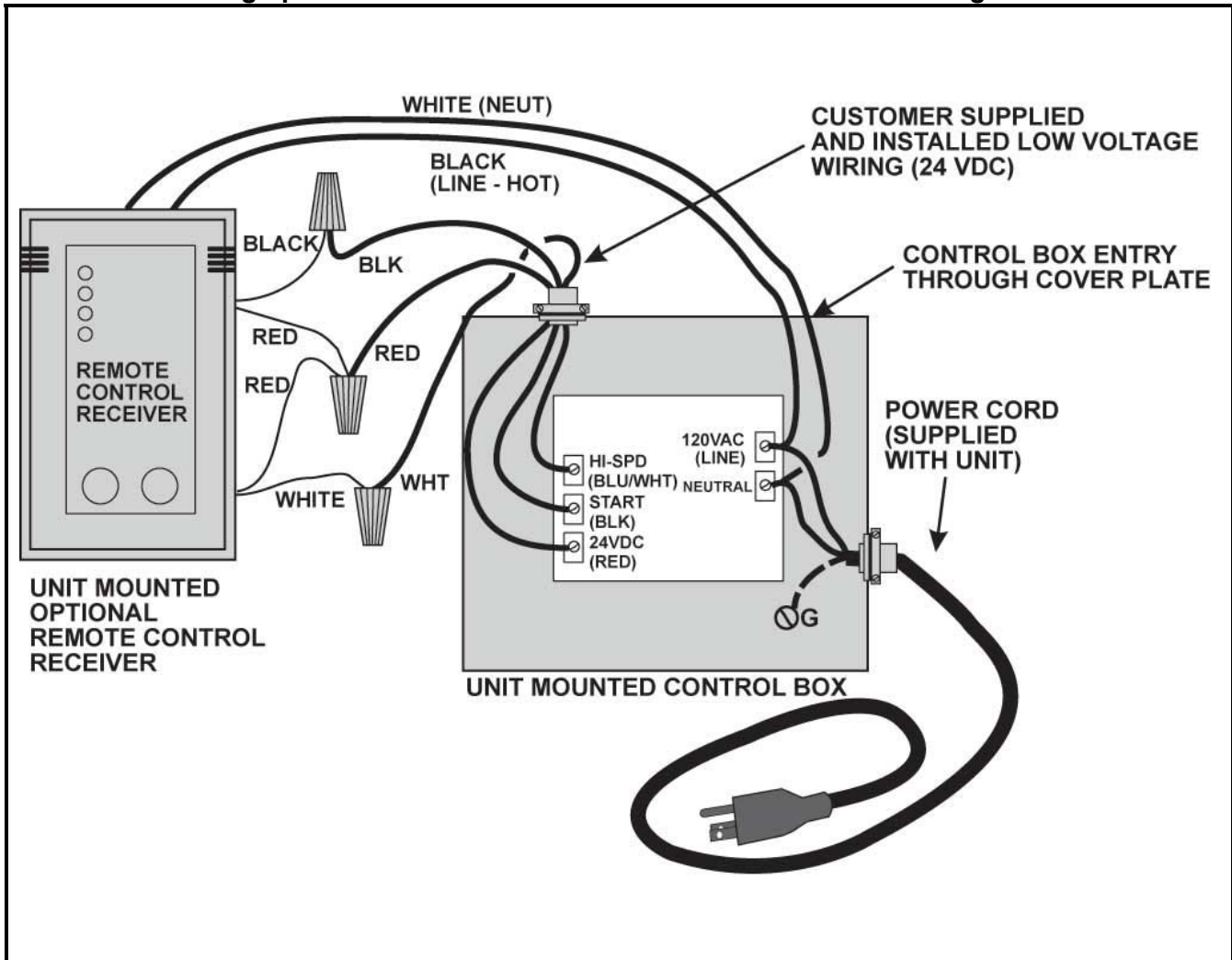
FIGURE 9 – Wiring optional remote control unit – Power AND control wiring shown
