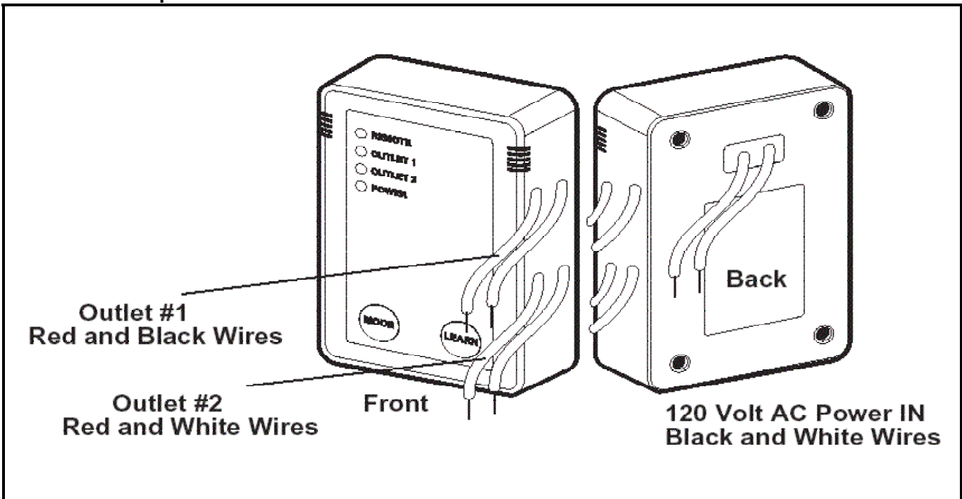
FIGURE 11 – Optional Remote Control Receiver.
