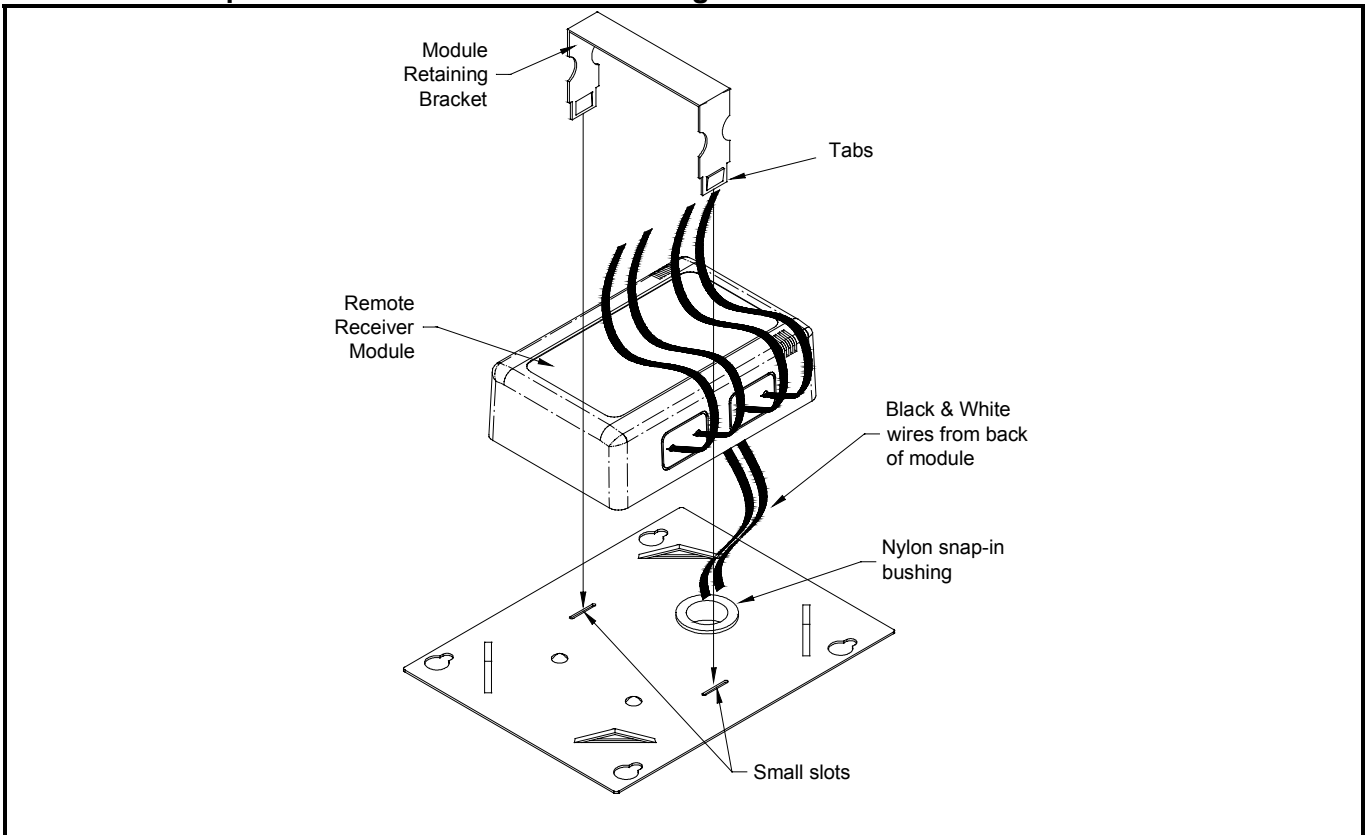
FIGURE 11 – Optional Remote Control Receiver.
