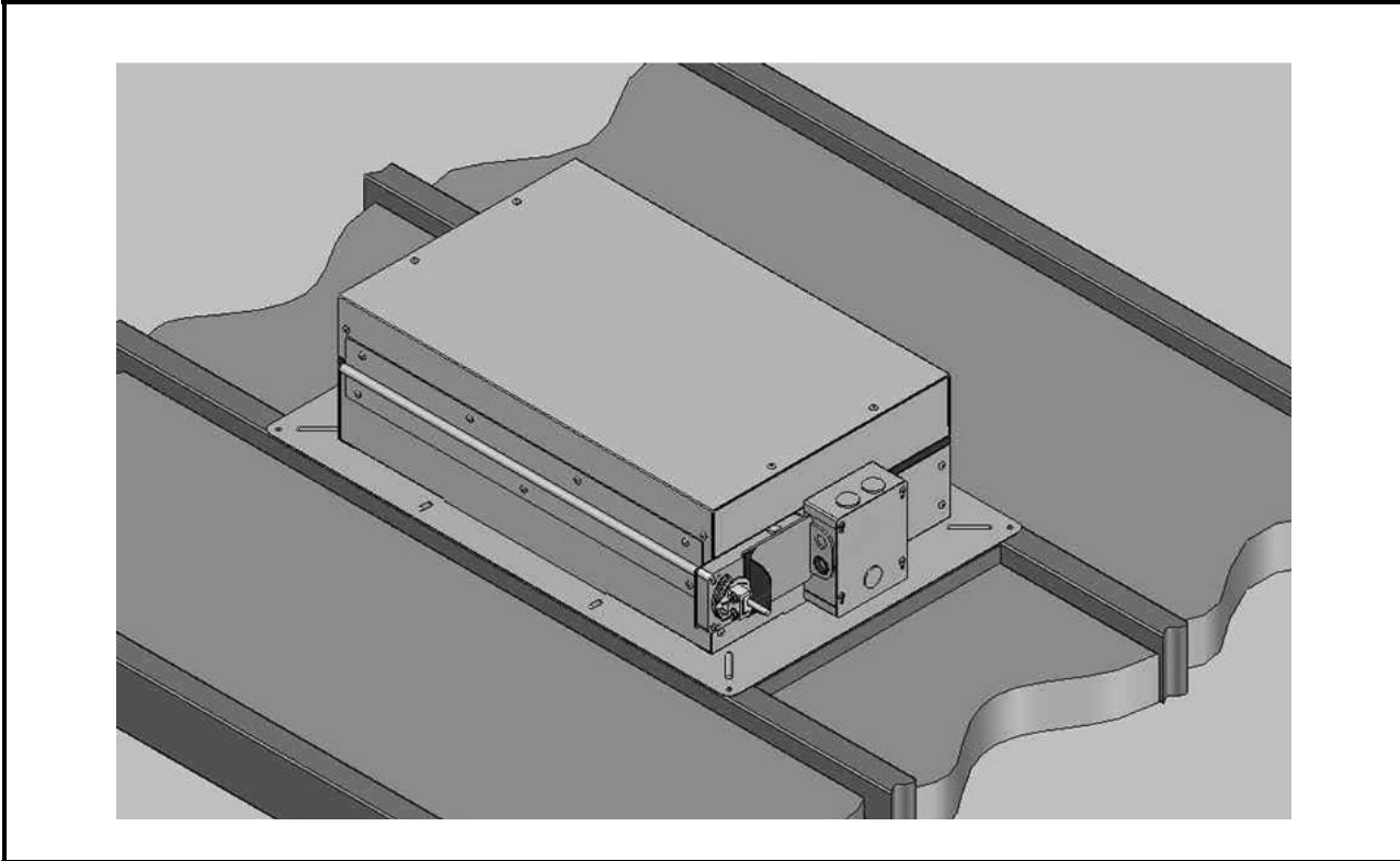
FIGURE 5 – Installed top (attic) view.
